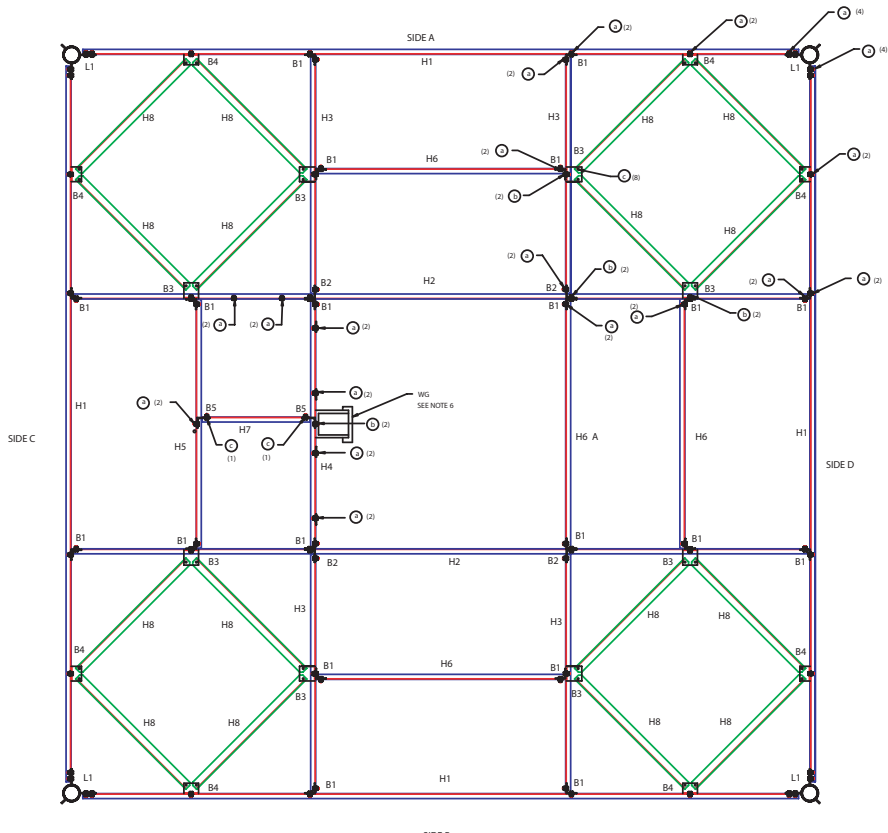
10 FT. SECTION HORIZONTAL LAYOUT
