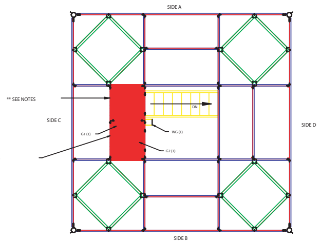
STAIR AND GRATING LAYOUT
